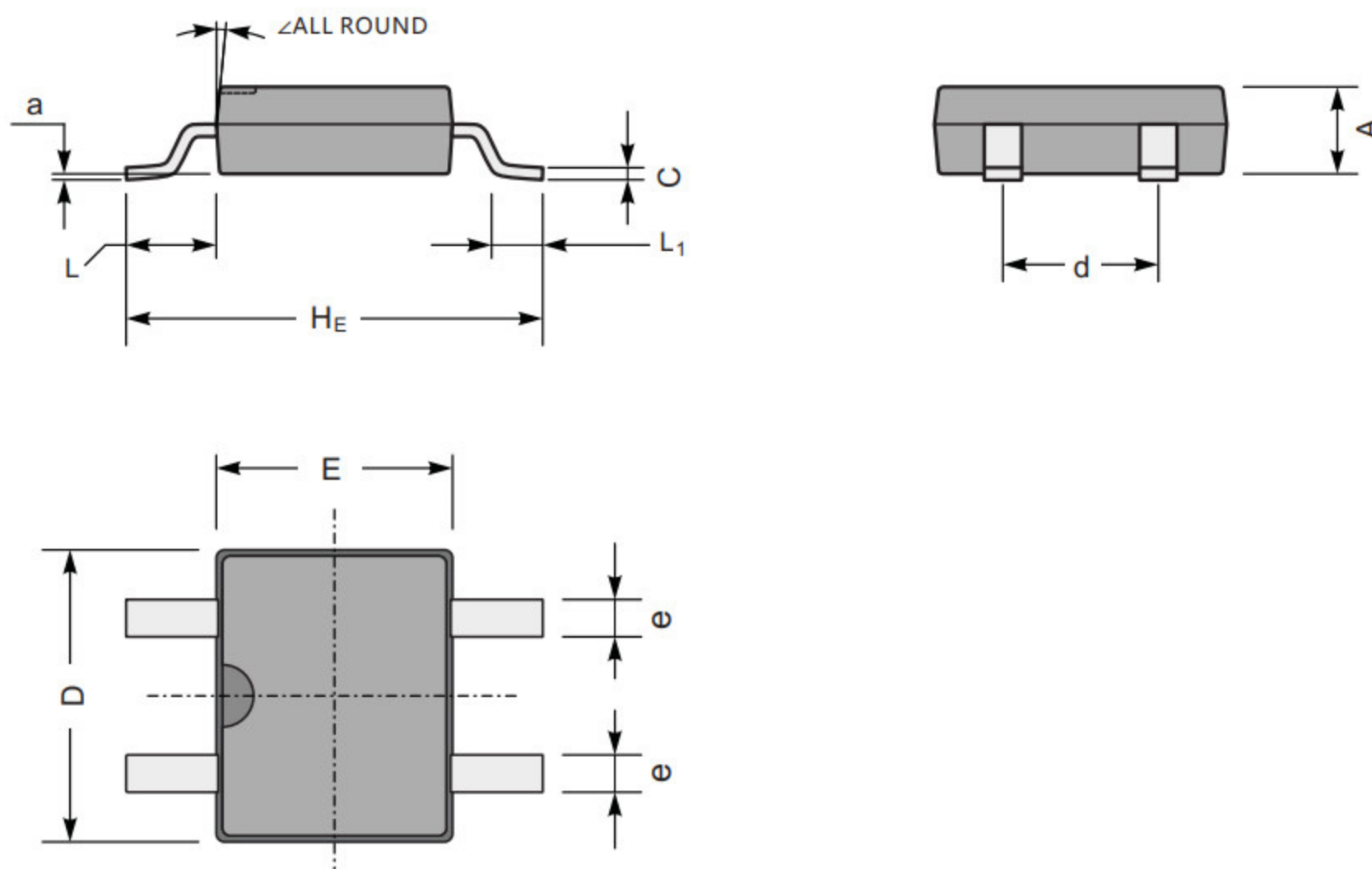
MBF mechanical data
